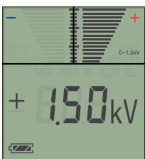
Wide Display The measured potential is displayed with a bar graph and values for quick confirmation
