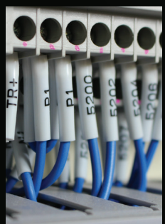
Vinyl Tubing with Half Cut Function
