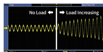
Motor Current
