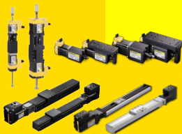
Ezi-ROBO ® CC-Link IE TSN Precise Actuator System
