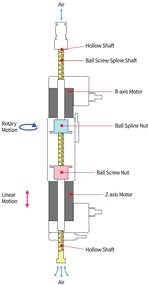
Ezi-ROBO VZR Product Structure
