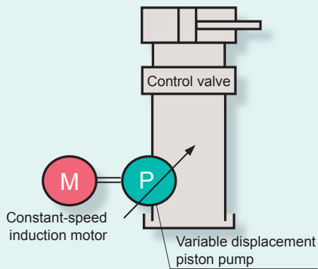
Conventional hydraulic system
