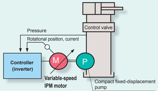
EcoRich R system
