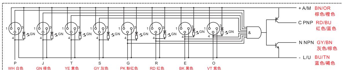
AJB8M8-3N-M16
