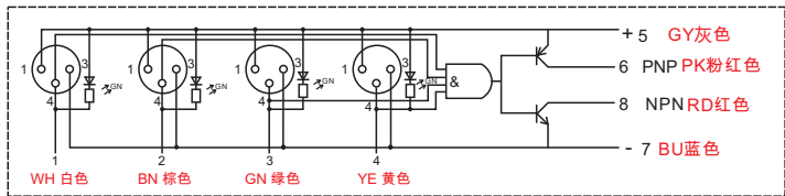
AJB4M8-3N-M12
