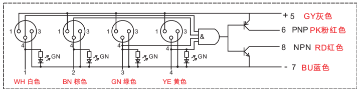
AJB4M8-3P-M12
