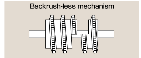
Backrush-less mechanism Divided worms catch the rack on lower jaw firmly. This mechanism enables not to loosen the wrench.
