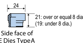
Side face of E Dies Type A
