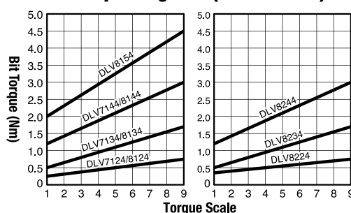
Torque Diagrams (for reference)
